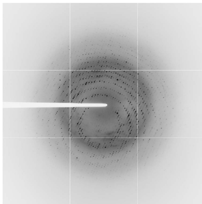
Figure 2 Diffraction image of a PhoRadA intein crystal. The image was prepared using the ADXV program ( http://www.scripps.edu/~arvai/advx.html ). The resolution at the edge of the image is 1.75 Å. The data were collected on the ESRF ID23-1 beamline using an ADSC Quantum Q315R detector.
