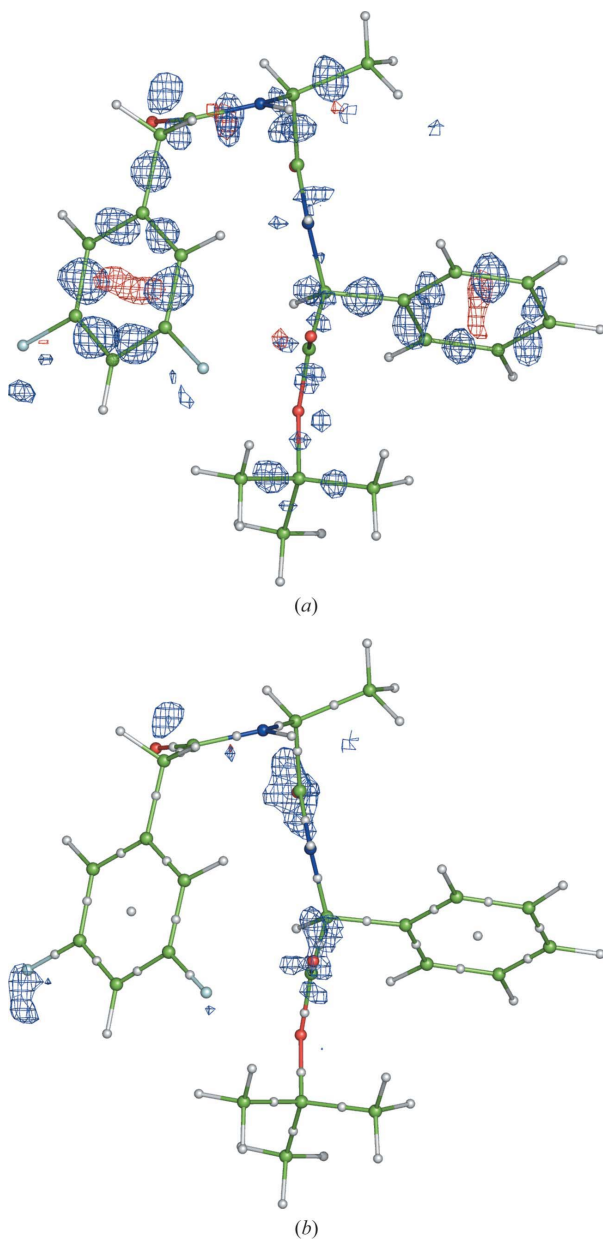
Figure 3 (a) Difference Fourier map at 0.11/–0.15 e Å –3 contour levels (in the electronic version of the paper, blue denotes positive and red negative) before modeling interatomic scatterers in PHENIX . (b) Difference Fourier map after IAS refinement at the same contour levels. The positions of the interatomic scatterers (at the centers of the bonds and phenyl rings) are marked as spheres of arbitrary radii, in addition to all atoms.
