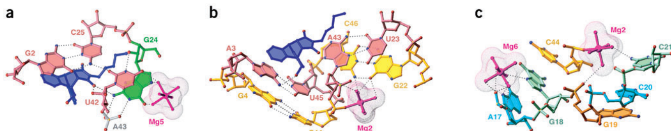
Figure 3 Structural elements of the Diels-Alder ribozyme-product complex. The view is rotated 180^\circ along the vertical axis relative to the schematic in Figure 1b . The color code is the same as in Figure 2 , unless specified otherwise. Oxygen, nitrogen and phosphorus atoms are, respectively, red, blue and yellow balls. Hydrogen bonds are dotted lines. Coordination bonds to Mg atom are magenta sticks. (a) RNA segment aligned above the product. The A43 backbone is silver. (b) RNA segment aligned below the product. (c) Structural motif highlighting splaying out of G18 and G19.
