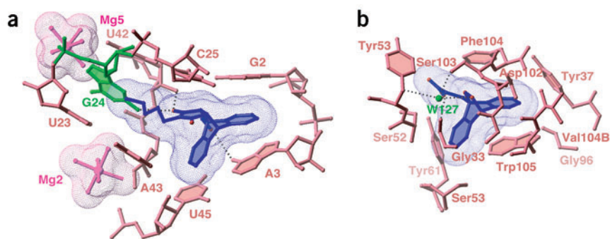
Figure 6 Comparison of the RNA and protein catalytic sites for the Diels-Alder reaction. The surface of the bound ligand is in mesh representation. (a) Catalytic pocket from the Diels-Alder ribozyme-product complex. (b) Catalytic pocket of the antibody catalyzing the retro-Diels-Alder reaction 41 (PDB entry 1LO2). Anchoring of the ligand is achieved through direct and water-mediated (W127) hydrogen bonds.
