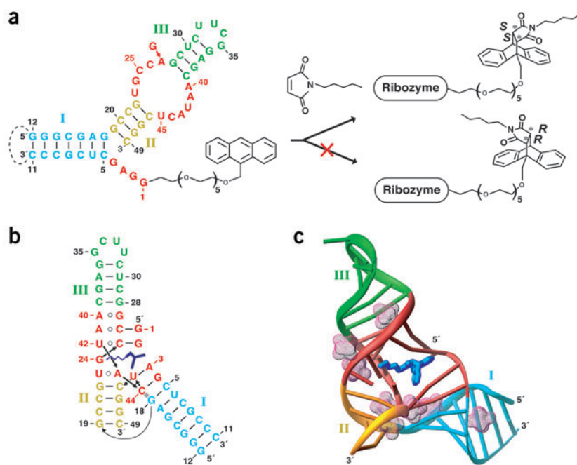
Figure 1 Secondary and tertiary folds of the Diels-Alder ribozyme. (a) Ribozyme secondary structure (left) with stems I–III in cyan, gold and green, respectively, and residues found invariant in the selection procedure in red. The same colors are used throughout this figure. The ribozyme consists of a 11-mer (G1–C11) HEG-linked with anthracene and a 38-mer (G12–C49). The dashed line indicates a loop present in the selected ribozyme and deleted in the bipartite system. The ribozyme-catalyzed Diels-Alder reaction between anthracene and N -pentyl maleimide results in formation of a single enantiomer of the complex (right). (b,c) Tertiary fold (b) and three-dimensional topology (c) in the crystal structure of the ribozyme–product complex. The RNA bases and bound product (blue) are cylinders in c . The backbone is depicted with a ribbon, whereas the hydrated Mg^{2+} cations are in a mesh representation.
