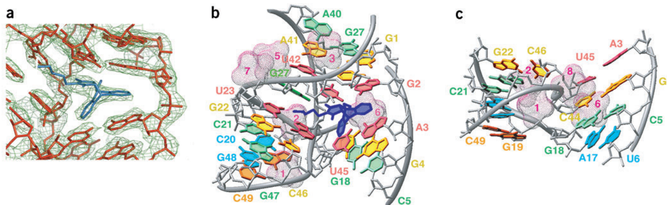
Figure 2 Details of the structure of the Diels-Alder ribozyme-product complex. (a) Final 2F_o - F_c electron density map (green), contoured at 1\sigma , for the cycloaddition product and surrounding RNA. The product (blue) and RNA (red), superimposed with the density, are from the refined model. (b) RNA tertiary structure surrounding the ribozyme catalytic pocket containing bound product. The product is blue, adjacent A3-U45 and U23•A43 base pairs and U42•(G2-C25) base triple are light red, G24 is green, with additional layers moving farther out from the pocket in gold (A41•(C26-G2), G22-C46 and C44-G4), light green (A40•G27, C21-G47 and G18-C5), cyan (C20-G48) and orange (G19-C49). The hydrated Mg^{2+} cations are in magenta-colored mesh. (c) Tertiary structure in the region of stems I and II. The RNA is slightly tilted compared with b to highlight the relative alignment of the stems. Individual base pairs and hydrated Mg^{2+} cations are shown as in b .
