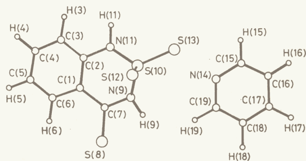
Figure 1. X-Ray structure of compound ( 1b )·C 5 H 5 N showing atom numbering scheme.
